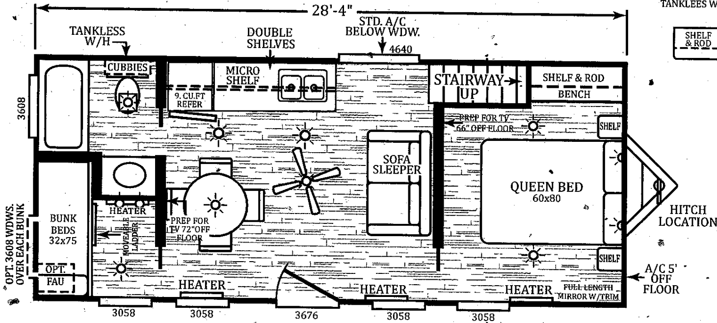
Model: CAN-1228 SL Size: 12' x 28' Description: Sleeps 6, Full Bath, Loft
