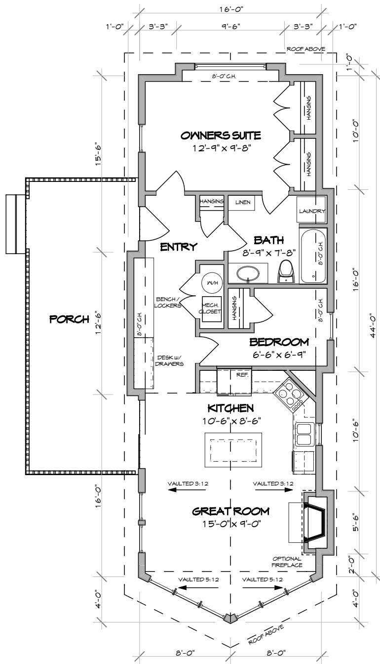
FLOOR PLAN - ESCAPE SCALE 1/8" = 1'-0"
