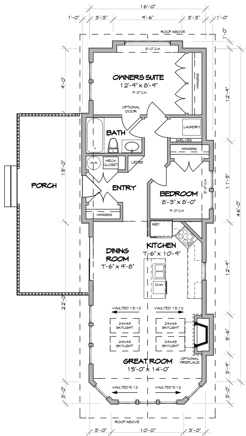
FLOOR PLAN - REFLECTION SCALE 1/8" = 1'-0" 16'-0" x 44'-0" 816 FEET SQ.
