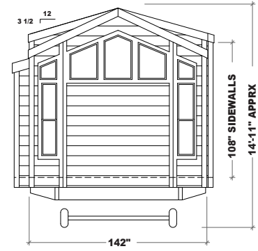
FRONT ELEVATION W/ALT LIVING ROOM
